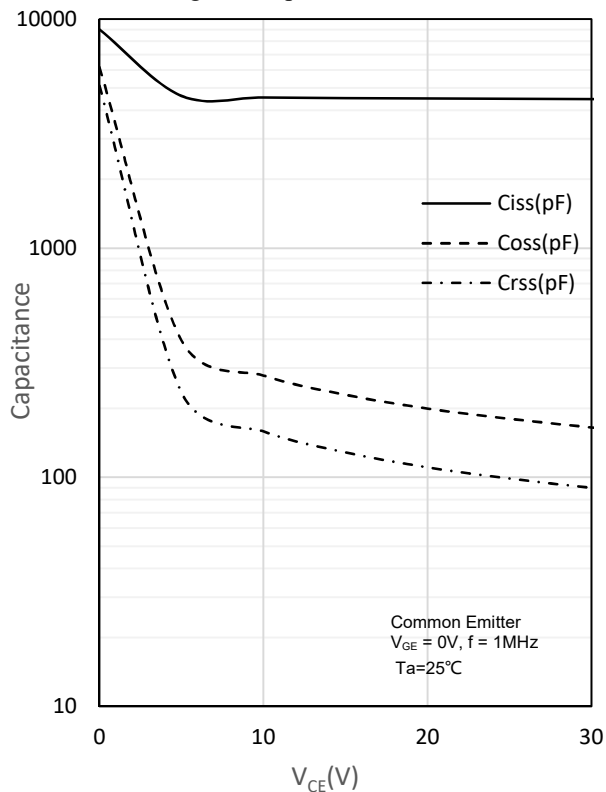
Fig. 12 Capacitance characteristics
